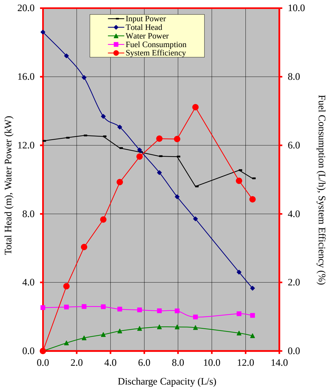
Figure 2. Performance characteristic curves of the MIYATA RBP 305 self-priming centrifugal pumpset
